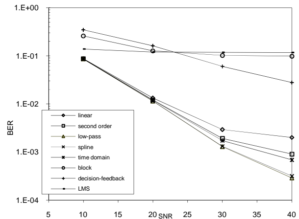
Fig. 4. BPSK (Channel 1) Rayleigh Fading
