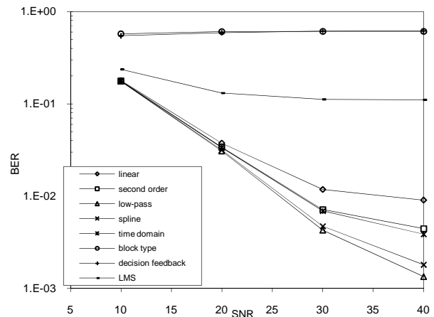
Fig. 5. QPSK (Channel 1) Rayleigh Fading
