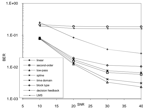
Fig. 6. 16QAM (Channel 1) Rayleigh Fading
